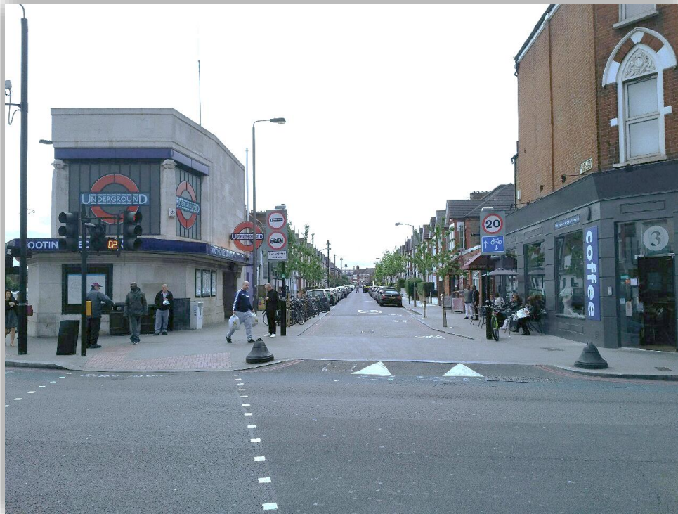
Example of bespoke 'blended footway' treatment, continuing the footway across a side road.
