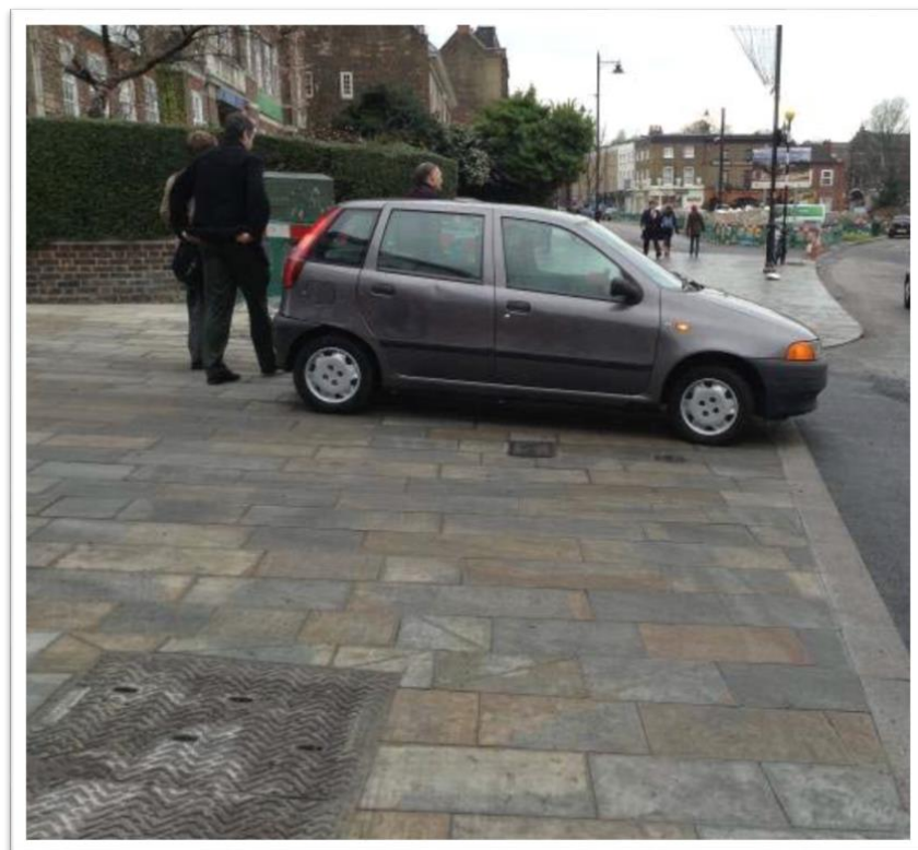
Example of bespoke 'blended footway' treatment, continuing the footway across a side road.
